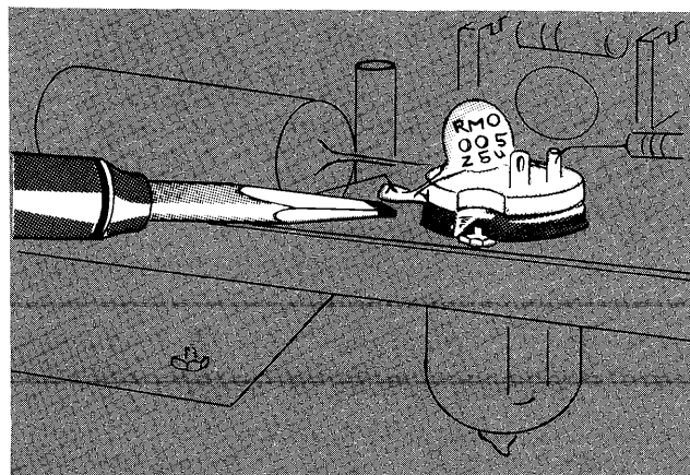
Fig. 5-4. Soldering to a terminal. Note the slight fillet of solder—exaggerated for clarity—formed around the wire.
