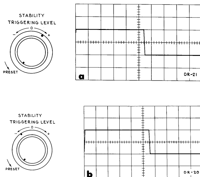
Fig. 2-5. Effect of the TRIGGERING LEVEL control when the TRIGGERING MODE switch is in the DC position. In the DC triggering mode, the setting of the TRIGGERING LEVEL control determines the elevation of the point on the graticule at which the display starts. (a) When the TRIGGERING LEVEL control is set in the + part of its range, the display starts at a point above the graticule horizontal center line. (b) When the TRIGGERING LEVEL control is set in the — part of its range, the display starts at a point below the graticule horizontal center line.
