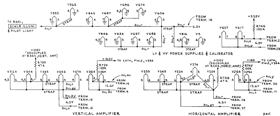
‡ TYPE 536 OSCILLOSCOPE
