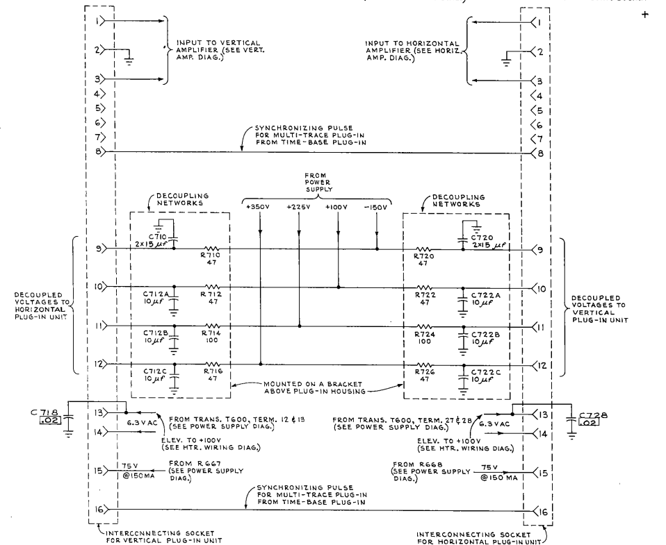
INTERCONNECTING SOCKET WIRING DIAGRAM
