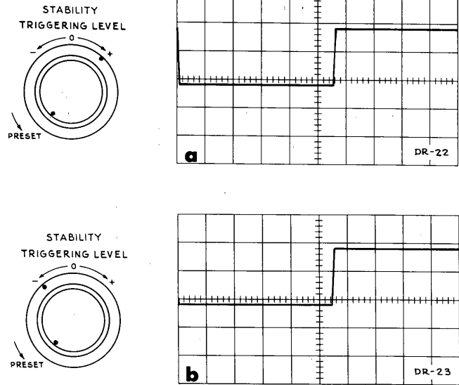
Fig. 2-3. Effect of the TRIGGERING LEVEL control when the TRIGGERING MODE switch is in the AC position. These drawings differ from those of Fig. 4 in that the black TRIGGER SLOPE knob is set at —EXT. This causes the display to start during the falling or negative-slope part of the waveform. (a) When the TRIGGERING LEVEL control is set in the + part of its range, the trace starts during the upper half of the waveform, just as it did in Fig. 4. (b) When the TRIGGERING LEVEL control is set in the — part of its range, the trace starts during the lower half of the waveform.
