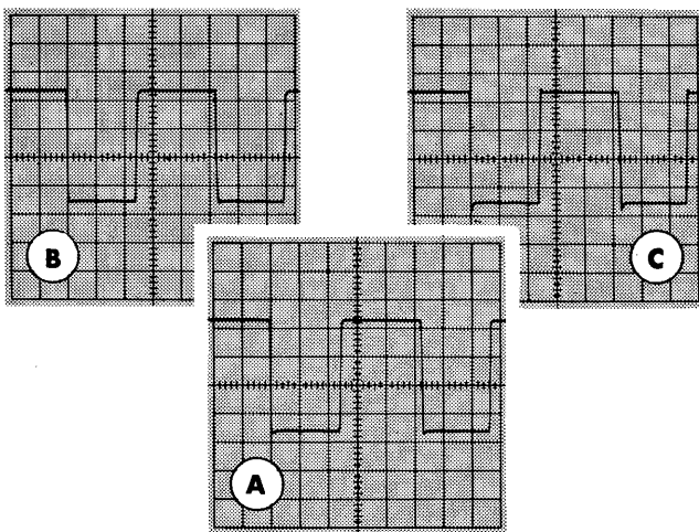
Fig. 6-7. Checking the high-frequency compensation of the vertical amplifier.
